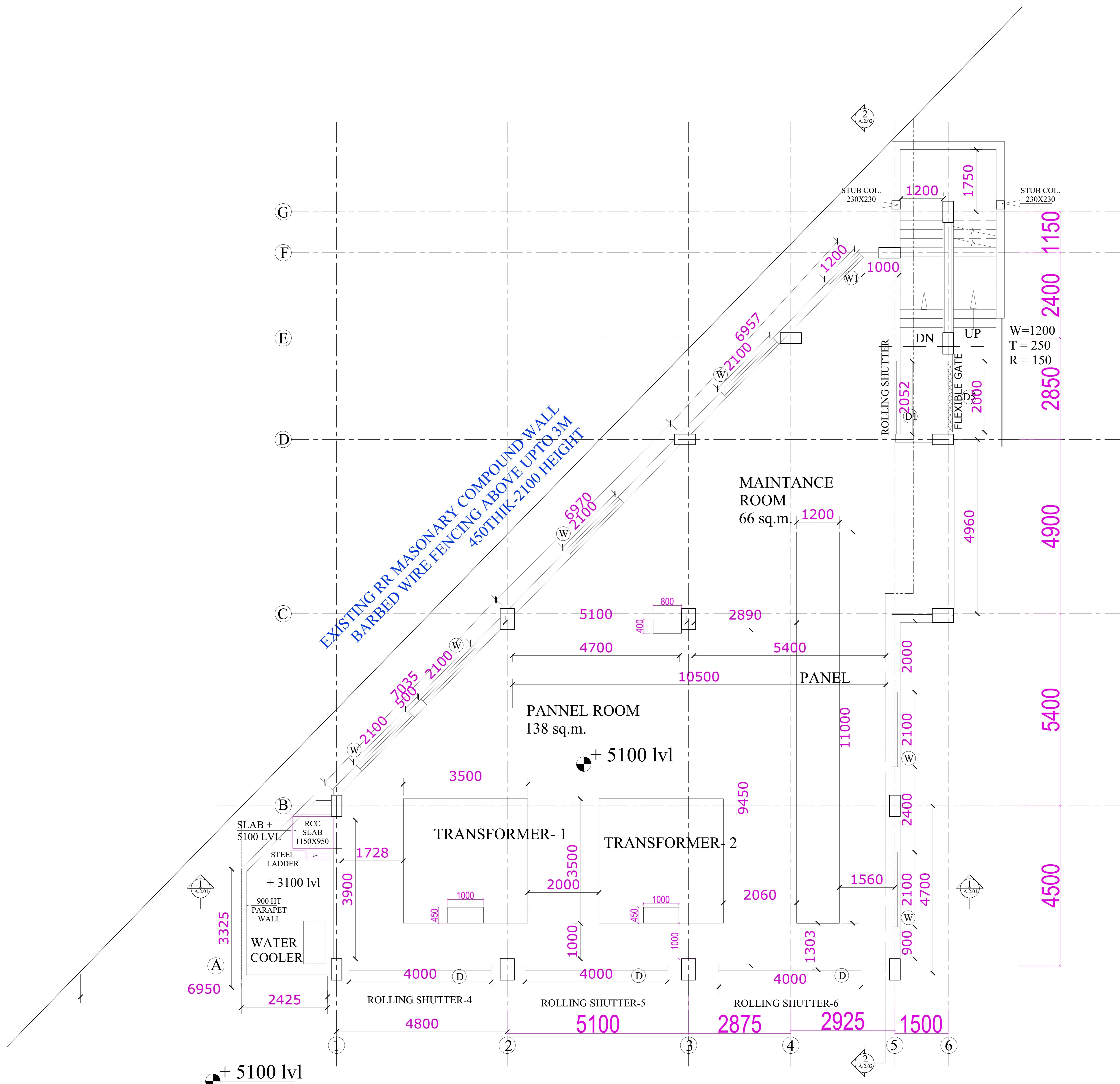
FIRST FLOOR PLAN
