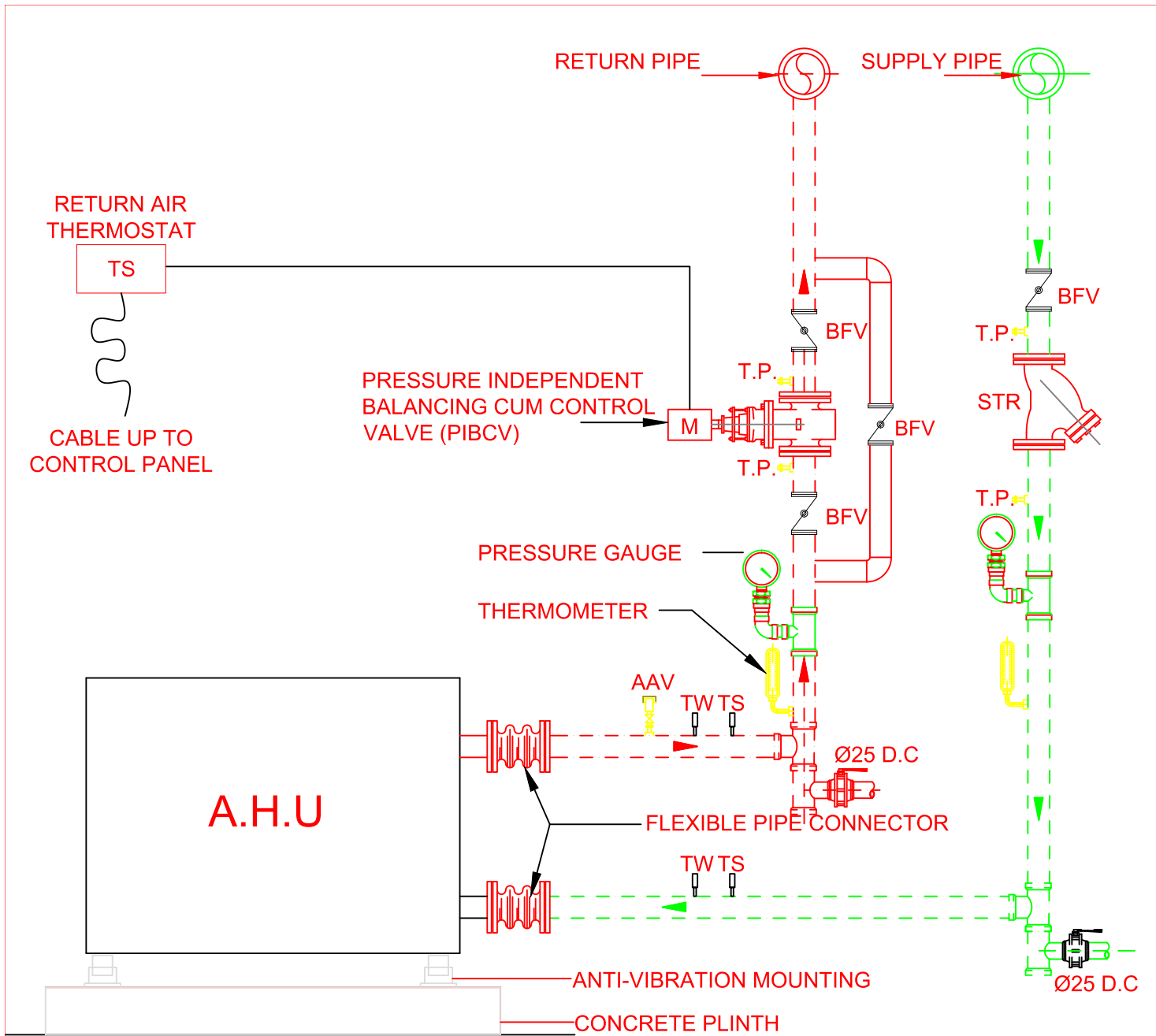
TYPICAL AHU PIPING CONNECTION DETAILS WITH PIBCV VALVE
