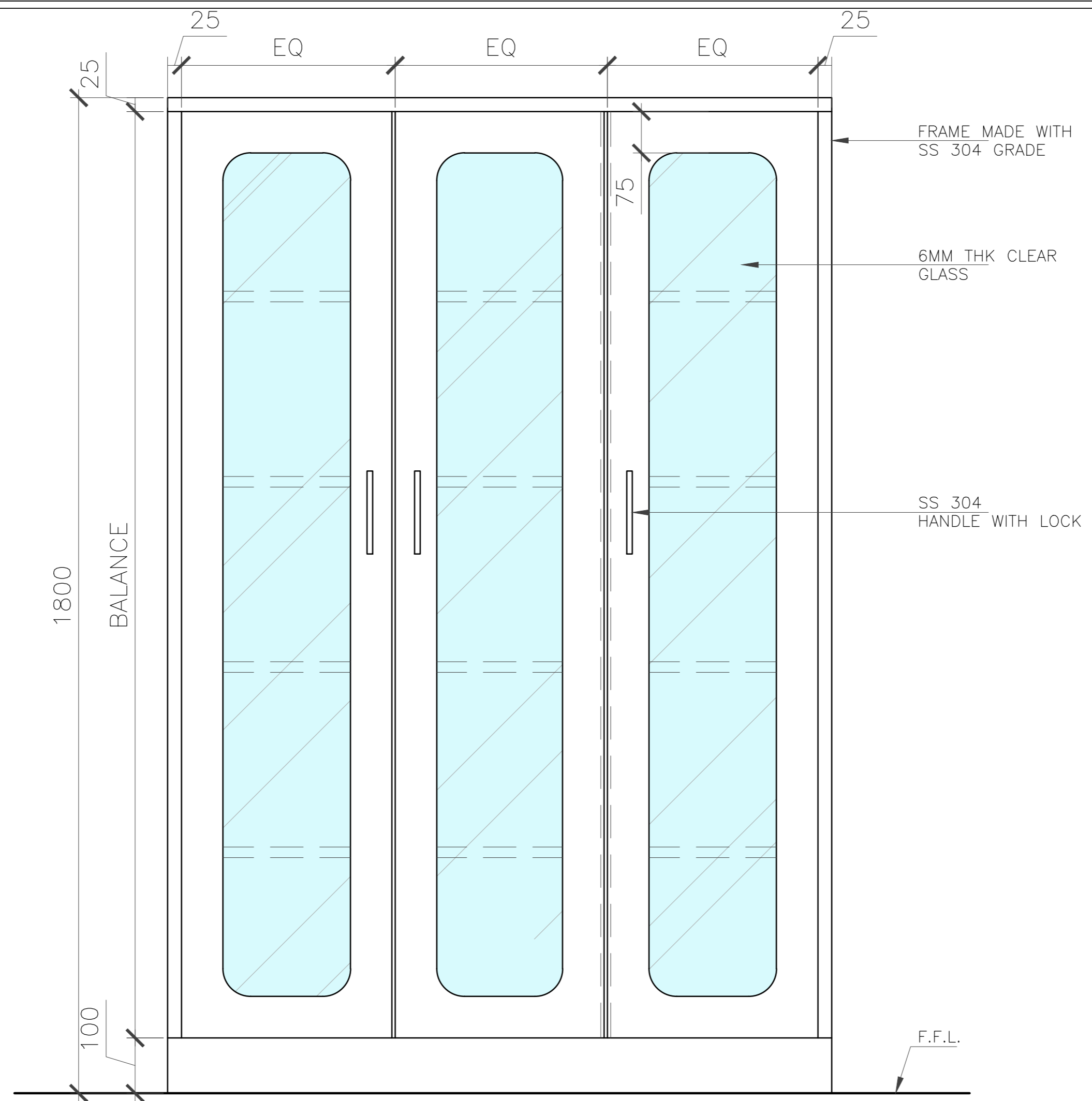
FRONT ELEVATION
